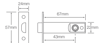
QS6002 Spring bolt
