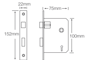
QS5757/2 two lever 57mm backset 57mm centre
