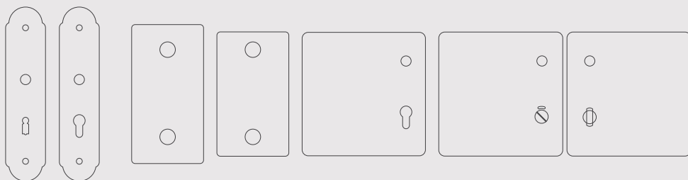
QS4489 KH 200x48x57mm CYL 200x48x60mm QS4487 190x100mm supplied with QS2205/1 QS4486 170x100mm supplied with QS2203/1 QS4485 170x170mm QS4485 with WC indicator
