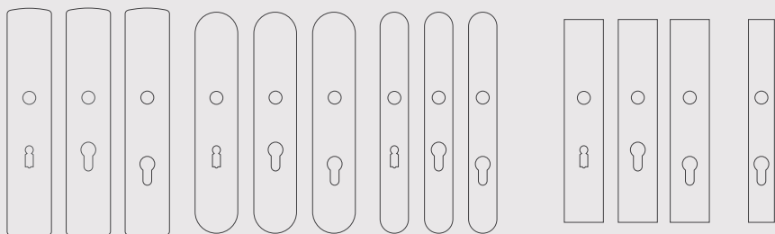
QS4482 KH 254x50x57mm CYL 254x50x60mm CYL 254x50x85mm QS4484 KH 245x45x57mm CYL 245x45x60mm CYL 245x45x85mm QS4483 KH 245x36x57mm CYL 245x36x60mm CYL 245x36x85mm QS4429 KH 225x40x57mm CYL 225x40x60mm CYL 225x40x85mm QS4428 CYL 225x28x85mm
