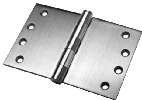
QS4412/1 100x150x3mm
